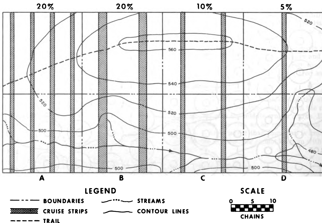
Figure 2-11. Strip method of estimating a stand of timber.
